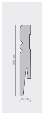
MP1005 100x15 mm SKIRTING 5905167674413 📏 2,42 m 📦 24,2 m 📦 847 m
