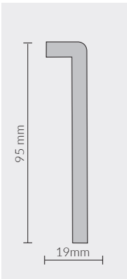
SO950 / WHITE 95x19mm SKIRTING 5905167817797
