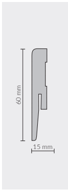
MP0602 60x15 mm SKIRTING 5905167754986 📏 2,42 m 📦 24,2 m 📦 1161,6m
