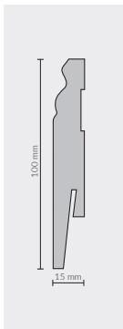
MP1003 100x15 mm SKIRTING 5905167674390 📏 2,42 m 📦 24,2 m 📦 847 m
