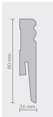
ML0802/ WHITE 80x16mm SKIRTING 5905167817858
