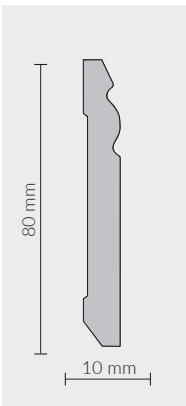
SO820 / WHITE 80x10mm SKIRTING 5905167817780
