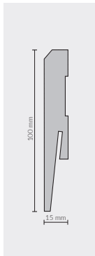
MP1001 100x15 mm SKIRTING 5905167674376 📏 2,42 m 📦 24,2 m 📦 847 m
